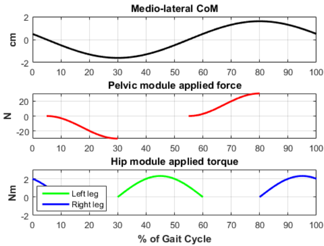
Figure 5. Desired force and torque reference trajectories for the pelvic module and the hip module with respect to the gait cycle. Medio-lateral force applied by the pelvic module induces lateral motion of the CoM and weight shifting onto the stance leg, followed by actuation of the swing leg by the hip module.
